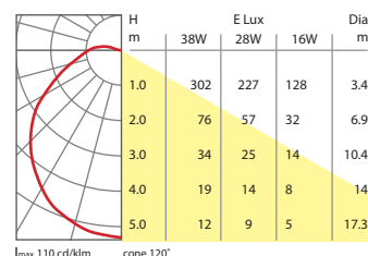
Corona 7 38W, 28W & 16W Opal Cover
