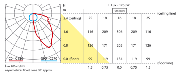
Illuminance on wall from luminaire mounted 1.2m from wall 1x55W TC-L
