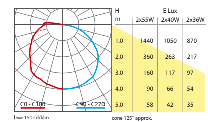
2x55W, 2x40W & 2x36W TC-L
